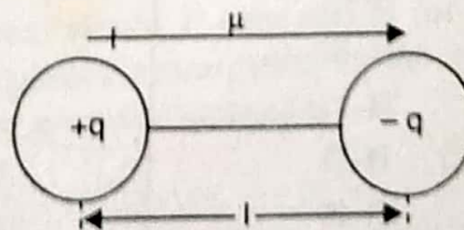
Fig. 8.2. Representation of dipole moment.
