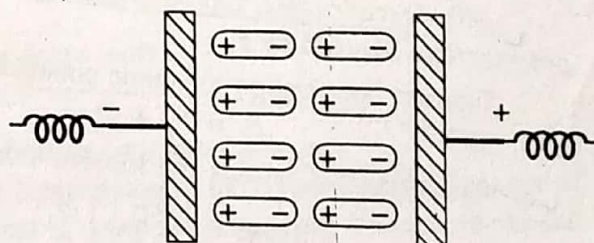
Fig. 8.5. If the polar molecules are stationary, they would orient at 180^\circ to the direction of electric field (i.e., perpendicular to the electric plates).
